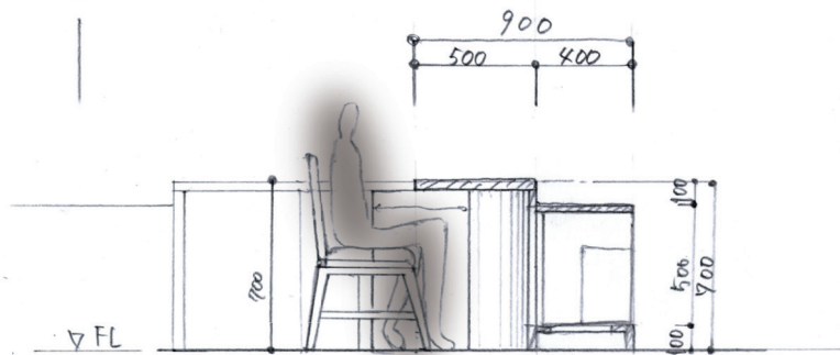
urniture detailed drawing
